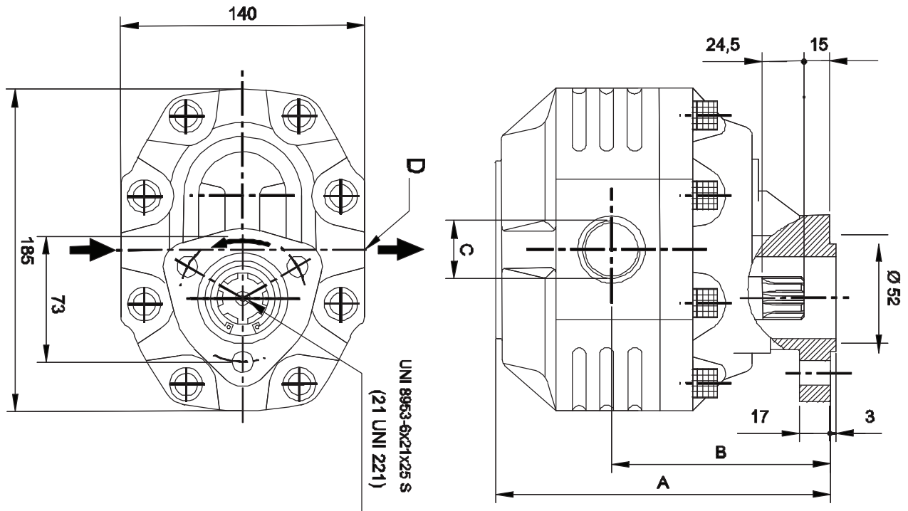
Gear pump BRT 4.Norma UNI
