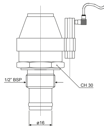
VISUAL-ELECTRICAL INDICATOR WITH "REED" CONTACTS
