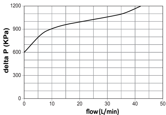
BY-PASS
