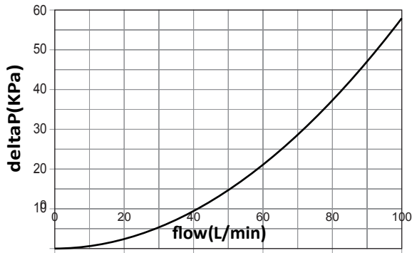
ΔP HOUSINGS
