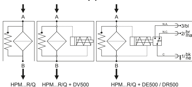
With By-pass
