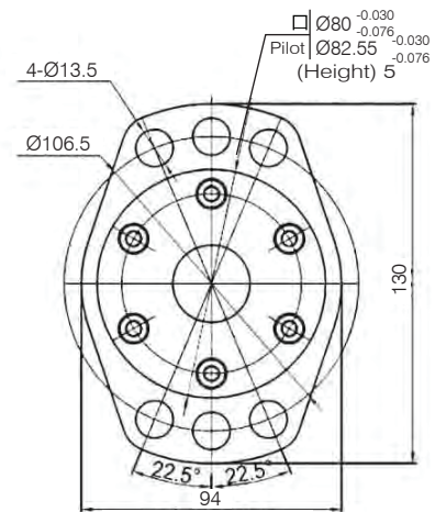
6 Bolt Flange
