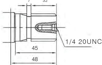
6D-Ø25.3X21.3x6.25 Recangle spline
