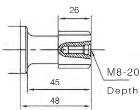
6D-Ø25X21.5x6 Recangle spline
