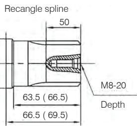
6D-Ø30X26X6
