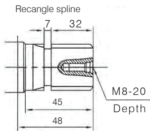
6D-Ø25.3X21.3x6.25 Recangle spline
