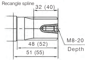
6D-Ø30X26X6
