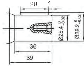
Ø25.4-6.35 Parallel
