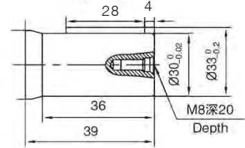
Ø30-8 Parallel
