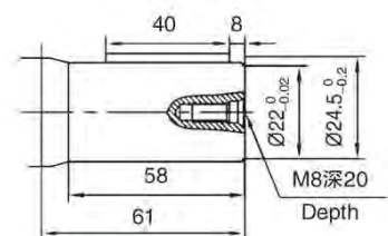
Ø22直轴平键6 Parallel
