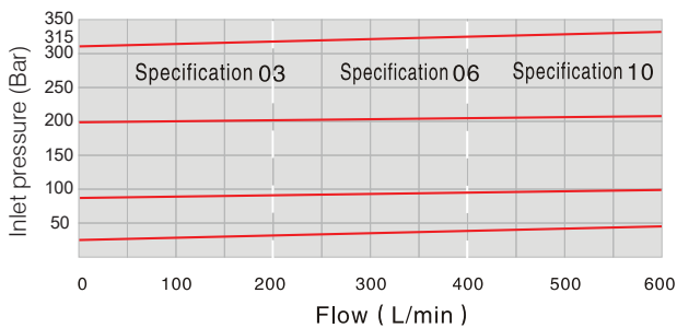
Inlet pressure in relation to the flow (A→B)
